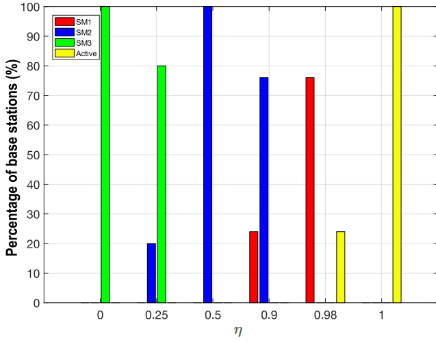
Fig. 2: States of the BSs for different values of \eta .
