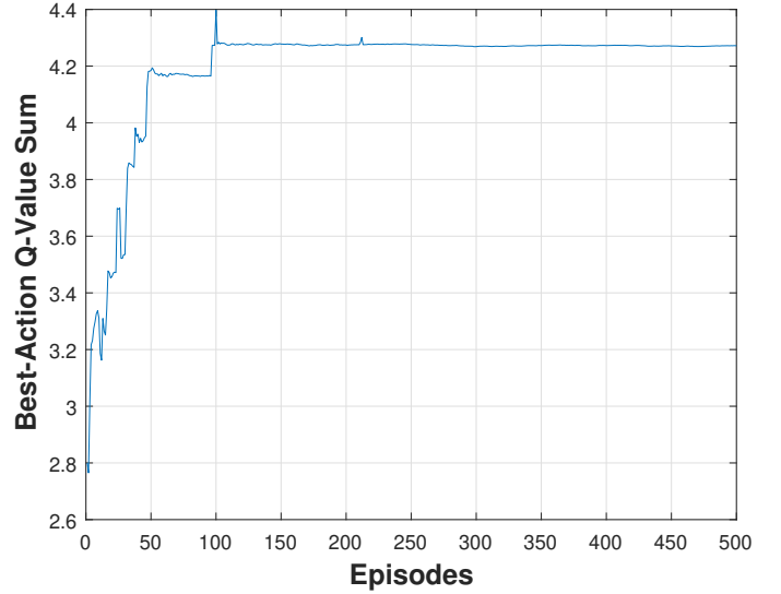
Fig. 1: Convergence of the Q-learning algorithm.
