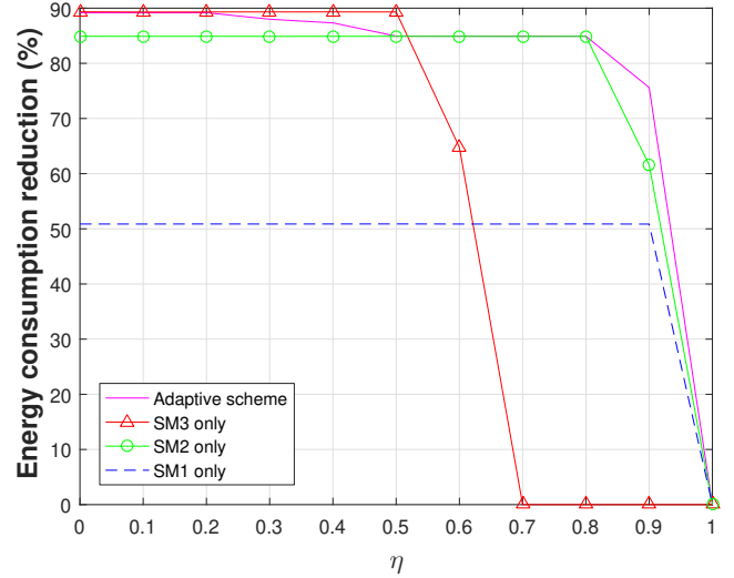
Fig. 5: Energy savings comparison between our proposed algorithm and the cases of using only one type of sleep mode.
